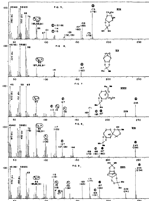
Fig. 5.—Mass spectrum of 2,3-O-isopropylidene-D-ribofuranose (XIV).
