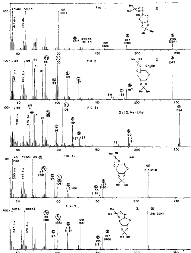
Fig. 1.—Mass spectrum of 1,2:5,6-di-O-isopropylidene-D-glucofuranose (V).
